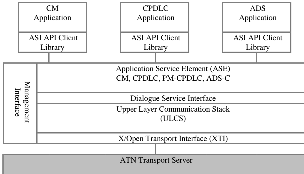
ATN Data Link Server Architecture
